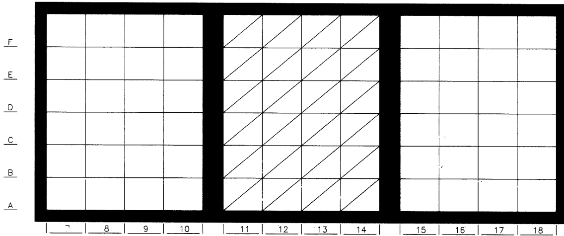
24 SINGLE DEPTH CRYPTS 24 DOUBLE DEPTH CRYPTS ELEVATION 301 24 SINGLE DEPTH CRYPTS
