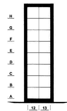
16 UNIT NICHE CABINET ELEVATION 814
